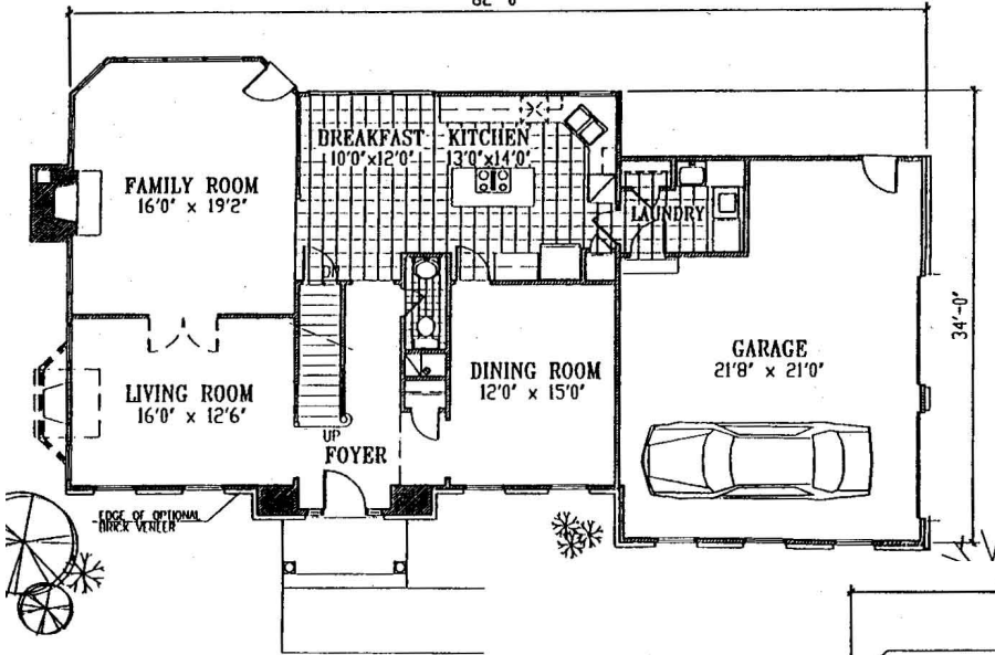
Lower Floor Plan Ceiling 9'
